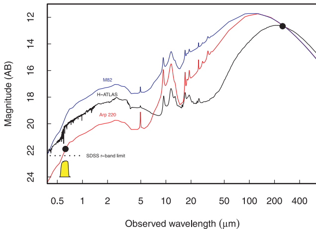
Figure 1. Templates for three galaxies showing the range of optical fluxes expected for galaxies which are at the SPIRE flux limit of S_{250} = 32 mJy at z = 0.5 , the limit of our study. The templates are for M82 (a typical starburst), an H-ATLAS template derived from our survey data by Smith et al. (2011b), and Arp 220, a highly obscured local ultraluminous infrared galaxy (ULIRG). The SDSS limit of r = 22.4 is shown as a horizontal dotted line and even a galaxy as obscured as Arp 220 is still visible as an ID to our optical limit at z = 0.5 . The yellow shape represents the SDSS- r -band filter which was used to compute the optical flux.
