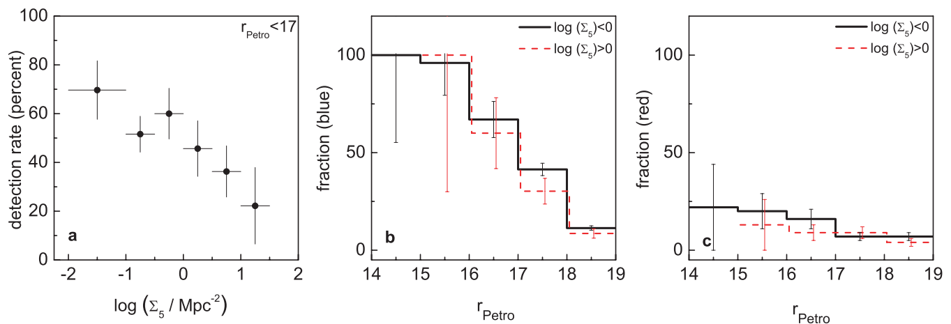
Figure 4. (a) The fraction of SDSS galaxies detected in H-ATLAS as a function of galaxy local density \Sigma_5 estimated using equation (2). (b) Histograms of the fraction of detected blue ( u - r \leq 2.2 mag) galaxies as a function of r -band magnitude. ‘The red dashed histogram’ includes galaxies in high density regions ( \log(\Sigma_5/\text{Mpc}^2) \geq 0 ) and ‘the black histogram’ includes those in low density regions ( \log(\Sigma_5/\text{Mpc}^2) < 0 ). (c) Same as in ‘b’ but for red ( u - r > 2.2 mag) galaxies.
