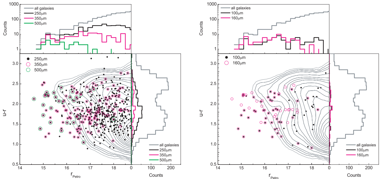
Figure 1. Colour–magnitude diagram of optically selected galaxies (grey contour lines) and their submillimetre counterparts with \text{Reliability} \geq 0.8 detected at \geq 5\sigma by SPIRE (left-hand panel) and PACS (right-hand panel). Horizontal and vertical histograms show the distribution of galaxy optical colour ( u - r ) and r -band magnitude ( r_{\text{Petro}} ), respectively. Colours represent: ‘grey’ all galaxies; ‘black’ sources with SPIRE 250 \mu\text{m} (left-hand panel) and PACS 100 \mu\text{m} (right-hand panel) detections; ‘pink’ sources with SPIRE 350 \mu\text{m} (left-hand panel) and PACS 160 \mu\text{m} (right-hand panel) detections; ‘green’ sources with SPIRE 500 \mu\text{m} detections.
