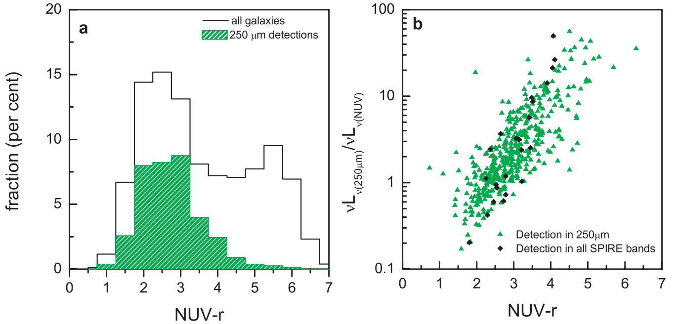
Figure 5. (a) NUV- r colour distributions for all the SDSS galaxies (black histogram) with available UV fluxes as well as those detected in 250 \mu\text{m} (green-shaded histogram). (b) The NUV- r versus \nu L_{250}/\nu L_{\text{NUV}} for galaxies with 250 \mu\text{m} detections (green triangles). Overlaid (black diamonds) are galaxies detected in all SPIRE bands.
