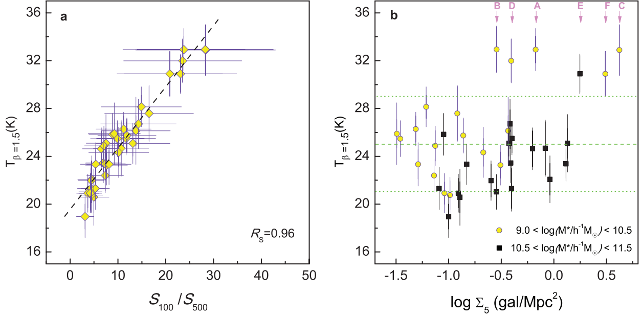
Figure 6. (a) Dust temperature versus submillimetre colour S_{100}/S_{500} . The dashed line shows the linear regression fit as described by equation (4). (b) Dust temperature as a function of the local density of galaxies, \Sigma_5 , for sources with \geq 3\sigma detections in SPIRE/PACS bands. The green dashed line intersects the y-axis at the mean temperature of the whole sample ( T \approx 25 K) while green dotted lines represent the standard deviation of the mean temperature. Circles and squares represent galaxies with low ( 9.5 \leq \log(M_*/h^{-2}M_\odot) \leq 10.5 ) and high ( 10.5 \leq \log(M_*/h^{-2}M_\odot) \leq 11.5 ) stellar mass, respectively. The SDSS images of objects marked as ‘A’ to ‘F’ (with ‘A’ having the maximum temperature) are shown in Fig. 7.
