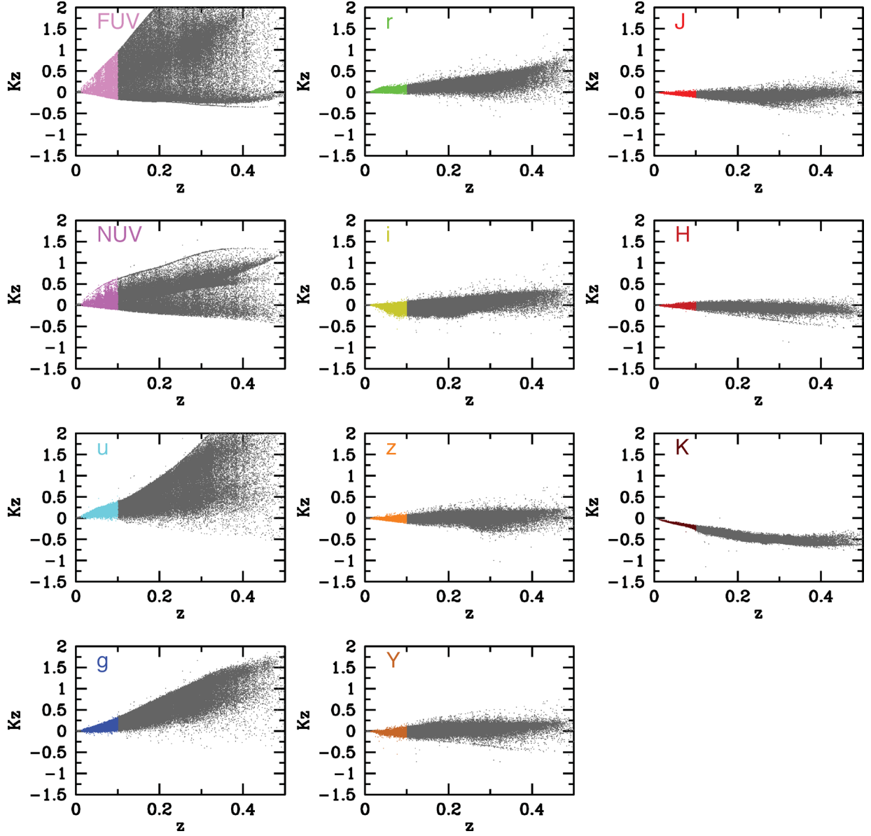
Figure 4. The k -corrections in each band for the full GAMA I sample as derived using \kappa\text{CORRECT} (v4.2), and indicating generally well-behaved distributions. Data in the redshift range 0.013 < z < 0.1 are shown in colour and represent the data used in this paper to derive the CSED.
