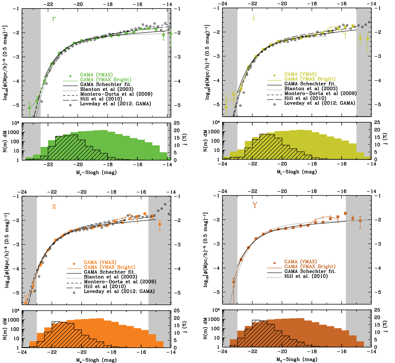
Figure 6. As for Fig. 5 but in the rizY bands.
