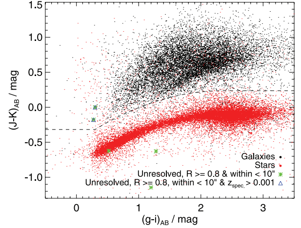
Figure 2. Colour–colour diagram for sources in the GAMA catalogue. We use the relationship of Baldry et al. (2010) to distinguish between unresolved sources (stars and QSOs) and galaxies. Those sources with stellar/QSO colours in the SDSS/LAS catalogue data over the GAMA 9h field are displayed in red, while those with galaxy colours are displayed in black. Objects with colours consistent with QSOs are located toward the upper left corner of this plot. Of the five R \geq 0.8 sources in our catalogue classified as unresolved, we find that three satisfy the GAMA colour selection criteria for being stellar, and so are potentially evolved stars, dust-obscured QSOs or debris disc candidates possibly indicative of a protoplanetary system (e.g. Thompson et al. 2010). The dashed line describes the first order star–galaxy separation locus (for more details see Baldry et al. 2010). The star–galaxy separation locus has been modified slightly from the Baldry et al. value due to the fainter magnitudes considered in our survey.
