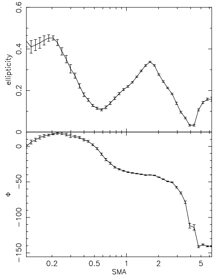
Figure 4. Ellipticity and P.A. as a function of semimajor axis of IRAF-fitted ellipses for run D at t = 400 .
