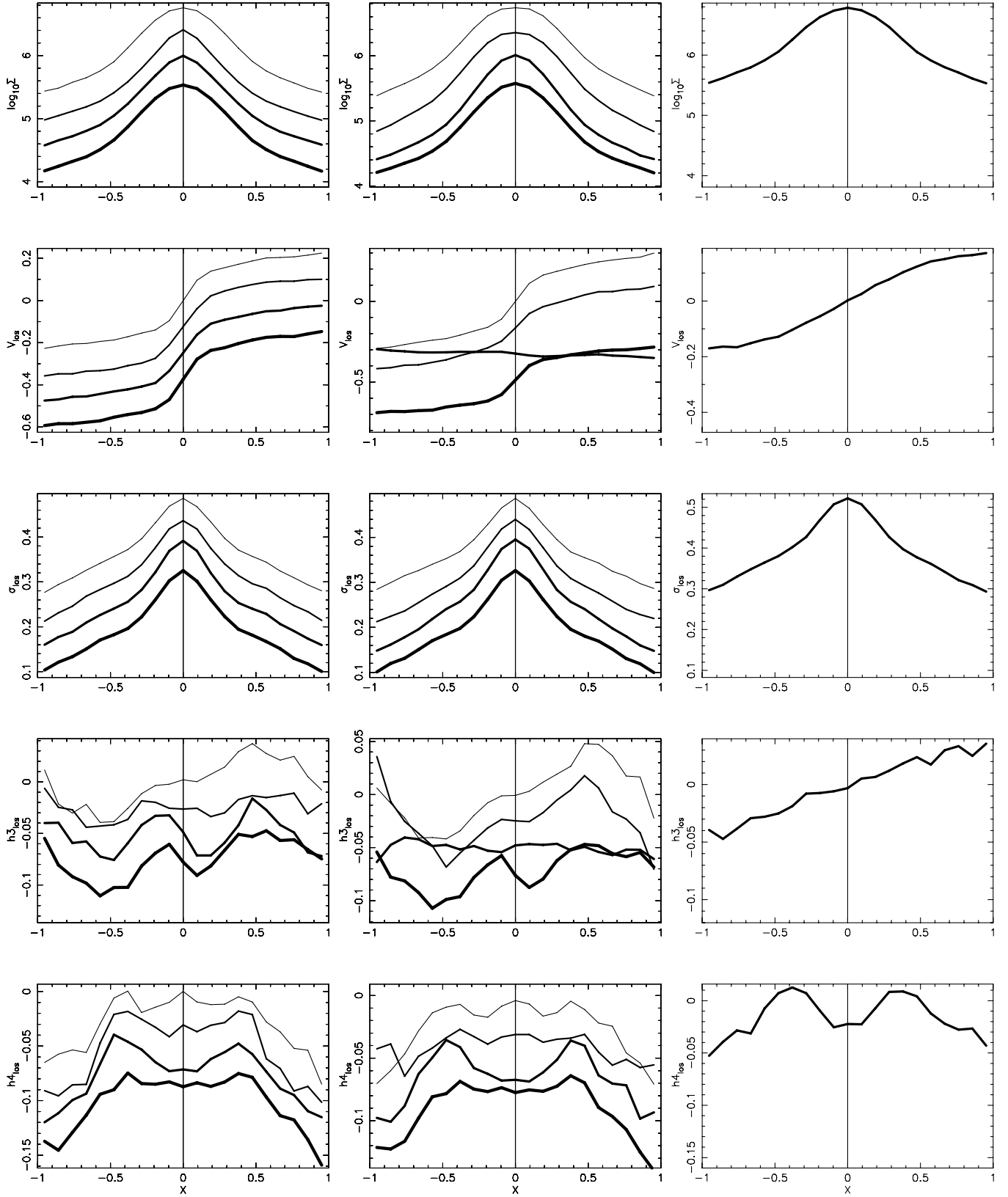
Figure 9. Evolution of slit profiles of runs D and S. From top to bottom panels: surface density, mean LOS velocity, velocity dispersion, h_3 , and h_4 . (a) Left column: slit profiles along the major axis of the primary bar in run D, as the secondary bar rotates through the primary one. In each panel the profiles from top to bottom with increasing line width, shifted by an arbitrary amount, represent t = 398 (two bars at 135^\circ ), t = 405 ( 90^\circ ), t = 412 ( 45^\circ ), and t = 415 ( \sim 0^\circ ), respectively. (b) Middle column: as in (a), but slits are along the major axis of the secondary bar in run D. (c) Right column: as in (a), but slits are along the major axis of the (single) bar in run S at t = 400 , which does not vary as the single bar rotates. The slit width is \sim 0.3 in all cases.
