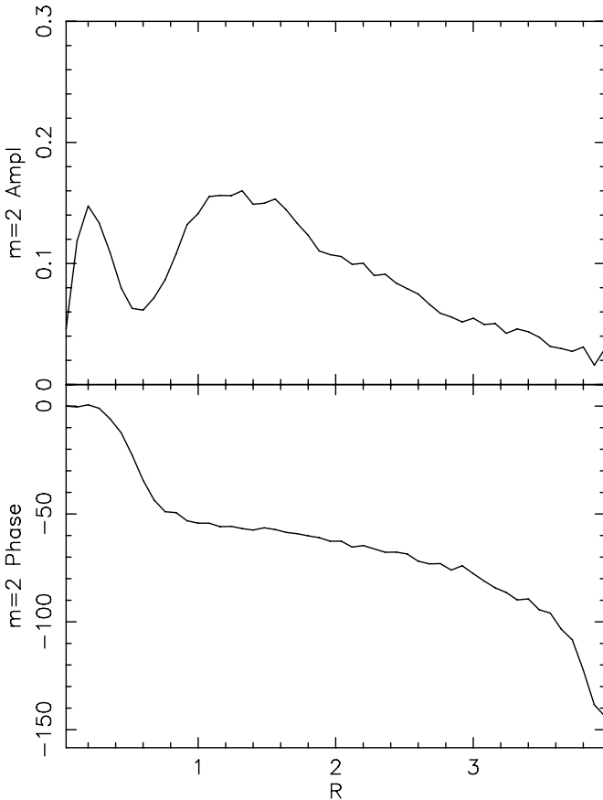
Figure 3. Radial variations of the m = 2 Fourier amplitude and phase of all particles for run D at t = 400 .
