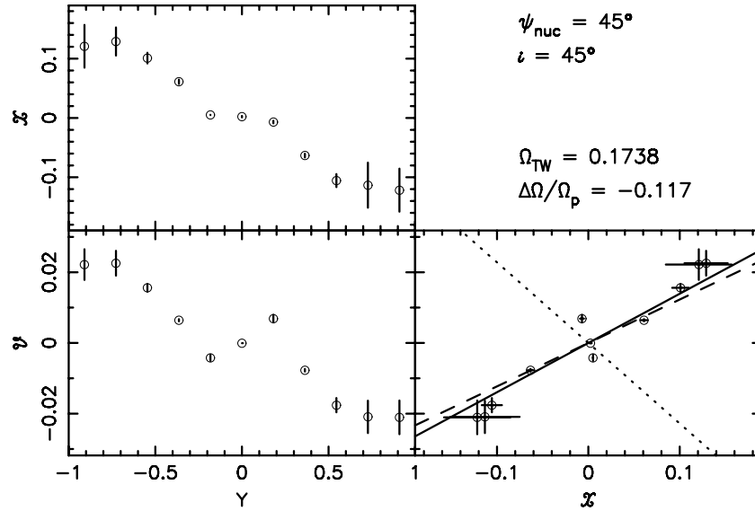
Figure 17. TW measurement for the full system of bulge+disk at t = 405 shown in Figure 2. The solid line is for \Omega_p while the dotted line is for -\Omega_p . The best-fit straight line to the points is shown by the dashed line. The relative weights of bulge particles (their “mass-to-light” ratio) have been adjusted to roughly reproduce \mathcal{X}(Y) in NGC 2950. This figure is to be compared with Figure 3 of CDA03.
