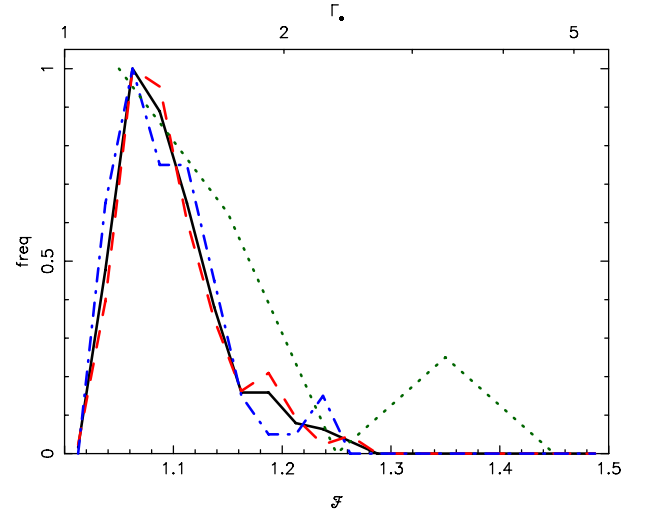
Figure 12. Distribution of \mathcal{F} for the various photometric samples. The dotted (green) line shows the classical bulges in the Graham (2003) sample. The remaining lines are for the Gadotti (2009) sample of classical bulges: the dashed (red) line is for unbarred galaxies, dot-dashed (blue) line for barred galaxies and solid (black) line for all galaxies. For ease of comparison, all distributions have been normalized to unit peak value. The top border is labeled by \Gamma_\bullet assuming \beta = 4.24 (Gültekin et al. 2009).
