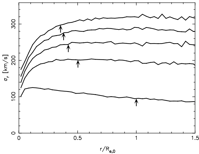
Figure 1. Evolution of \sigma_r , the radial component of the velocity dispersion in spherical coordinates, for the bulge particles in the R_d/R_{e,0} = 1 case. The profiles are at D/B = 0, 5, 10, 15 , and 20 , in increasing order. The arrows indicate R_e in each case.
