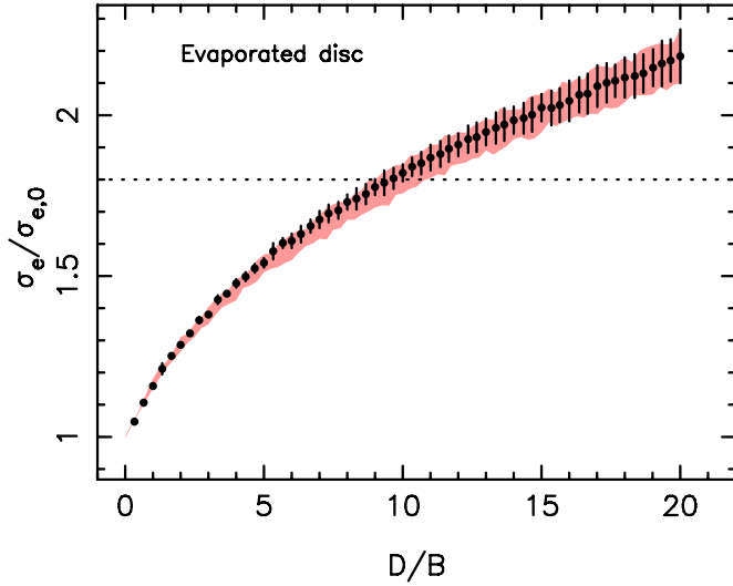
Figure 3. Evolution of \sigma_e in the R_d/R_{e,0} = 1 model as the disk is grown (red shaded region) and subsequently evaporated (black points with error bars). The dotted horizontal line indicates \sigma_e/\sigma_{e,0} = 1.8 for which \Gamma_\bullet = 10.5 if \beta = 4 . (A color version of this figure is available in the online journal.)
