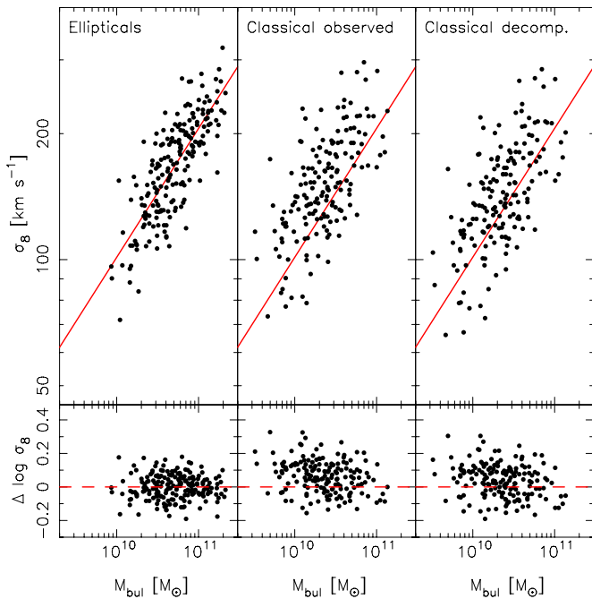
Figure 7. Distributions of ellipticals and classical bulges, taken from Gadotti (2009) and Gadotti & Kauffmann (2009), in the \sigma_8 – M_{\text{bul}} plane. Left: elliptical galaxies. Center: classical bulges in unbarred galaxies. Right: the same sample as in the central panel, but using the decompressed values for \sigma_8 obtained by applying Equation (9). The (red) solid lines in each of the upper panels show the best fit to the ellipticals: \Delta \log \sigma_8 = \log \sigma_8 - \log \sigma_{8,\text{fit}} , where \sigma_{8,\text{fit}} is the \sigma_8 value from the fit to the ellipticals of a given mass. (A color version of this figure is available in the online journal.)
