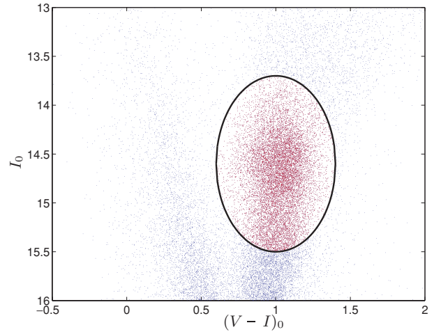
Figure 2. Extinction-corrected CMD for stars in the OGLE-II field 1. The ellipse defines the selection criteria for RCG stars based on colour and magnitude, see text. Sample stars are also required to have proper motion errors s_{l,b} < 1 \text{ mas yr}^{-1} and total proper motion \mu < 10 \text{ mas yr}^{-1} .
