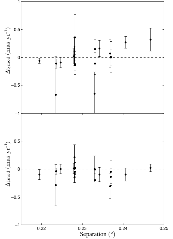
Figure 11. Difference between model proper motion dispersions for pairs of fields with separations less than 0^{\circ}25 .
