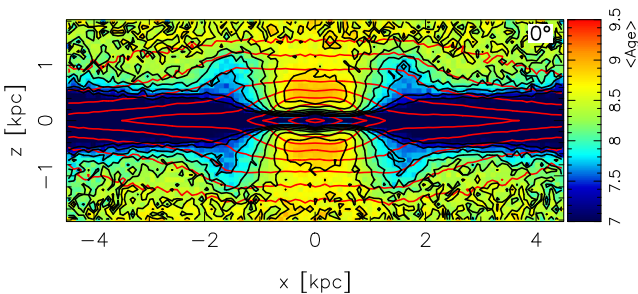
Figure 27. Map of \langle \text{age} \rangle (black contours and colours) and surface density (red contours) in the star-forming simulation seen edge-on with the bar side-on.
