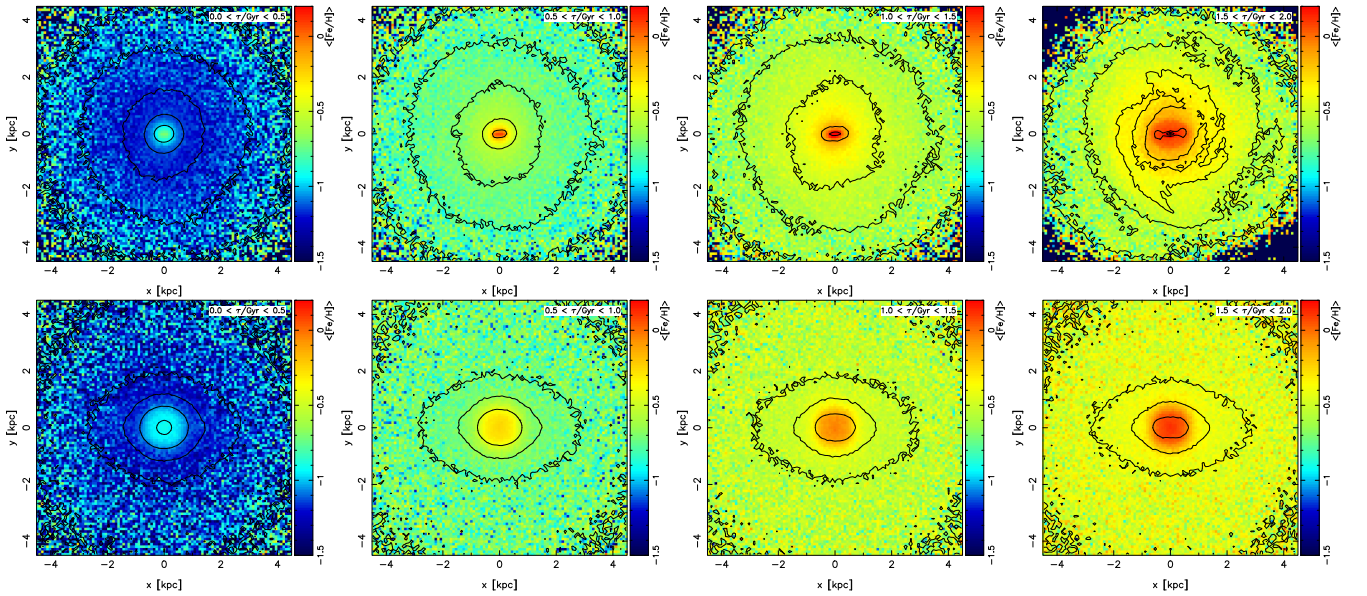
Figure 11. Maps of \langle[\text{Fe}/\text{H}]\rangle at t = 2 Gyr (top row) and t = 10 Gyr (bottom row) for different \tau populations as indicated at the top right of each map (from left to right, 0.0 \leq \tau/\text{Gyr} \leq 0.5 , 0.5 \leq \tau/\text{Gyr} \leq 1.0 , 1.0 \leq \tau/\text{Gyr} \leq 1.5 and 1.5 \leq \tau/\text{Gyr} \leq 2.0 ), in the star-forming simulation. The colour scale, indicated by the wedge beside each map, is common to all panels and spans -1.5 \leq [\text{Fe}/\text{H}] \leq 0.2 . Contours indicate the surface density of the different populations. The metallicity of populations rises rapidly with \tau .
