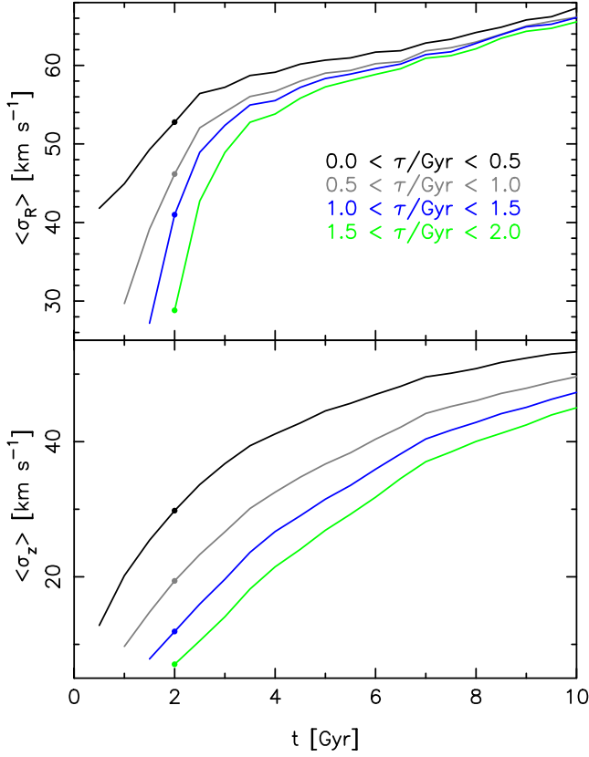
Figure 10. The evolution of \langle\sigma_R\rangle (top), and \langle\sigma_z\rangle (bottom) in the star-forming simulation. The different \tau populations are indicated in the top panel. Averages are taken over the radial range 1.5 \leq R/\text{kpc} \leq 3 . Note that at 2 Gyr (marked by the filled circles), as the bar starts forming, the radial and vertical dispersions increase with \tau .
