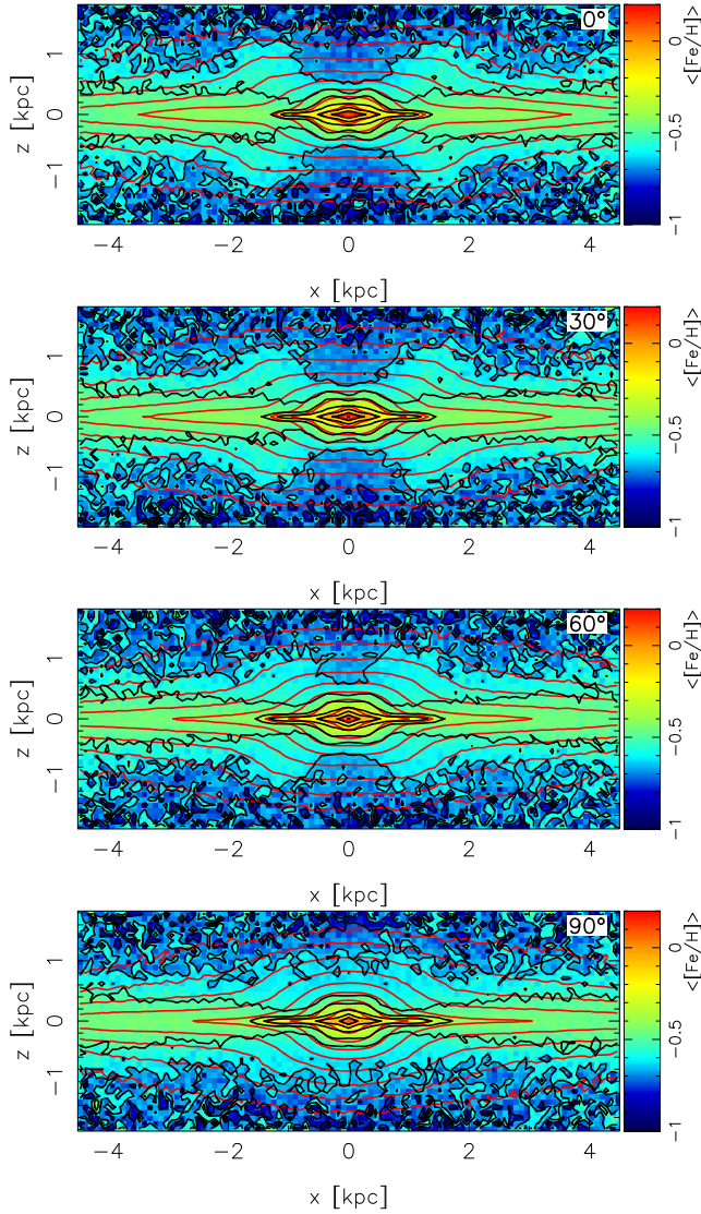
Figure 26. Maps of \langle [Fe/H] \rangle (black contours and colours) and surface density (red contours) in the star-forming simulation seen edge-on with the bar side-on (top), end-on (bottom) and two intermediate orientations (middle two panels). The bar’s orientation is indicated in the top right of each panel. These maps predict the trends in the metallicity distribution of external B/P-bulge galaxies.
