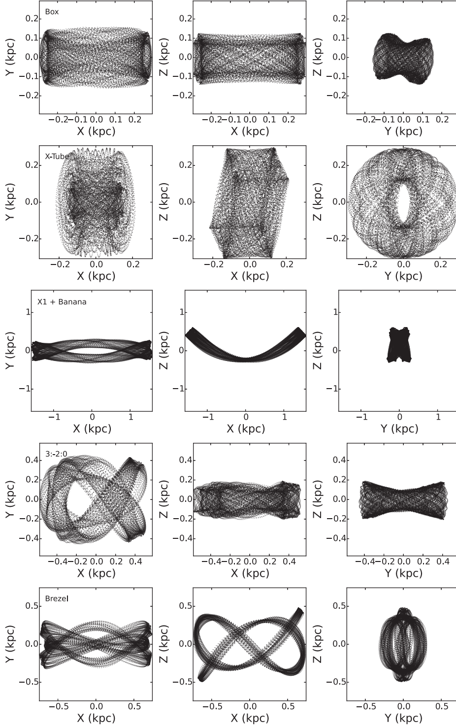
Figure 6. Three different projections of five different orbits in Model A. From the top to bottom: a box orbit, an x -tube orbit, a banana( x1v1 ) orbit ( 2:-2:1 ), a fish/pretzel orbit ( 3:-2:0 ) and a brezel orbit ( 3:0:-5 ).
